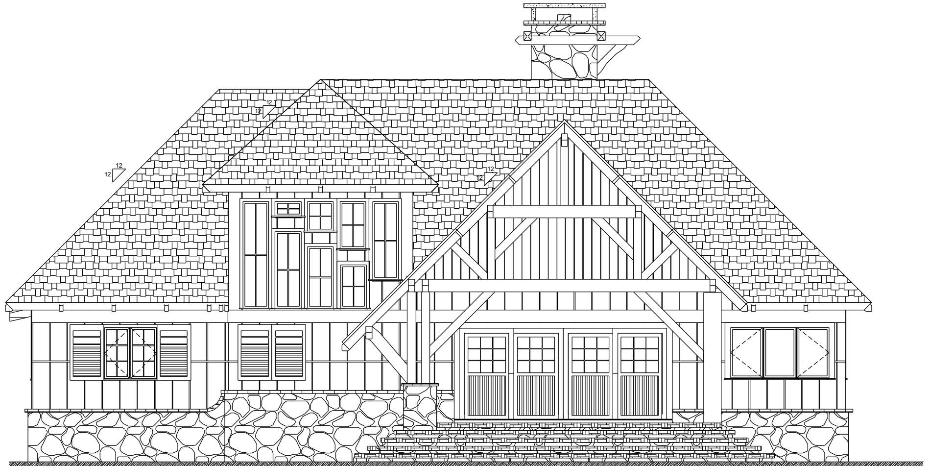
FRONT ELEVATION
